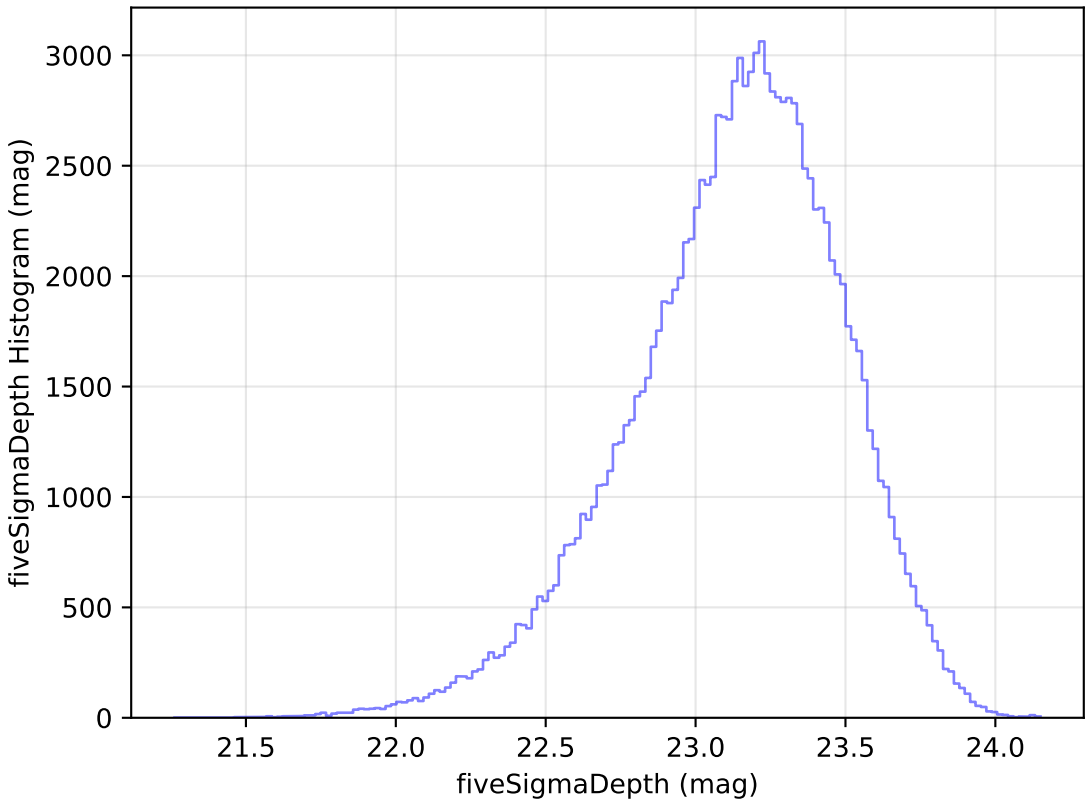
weather_cloudso6v3.4_10yrs u: fiveSigmaDepth Histogram
