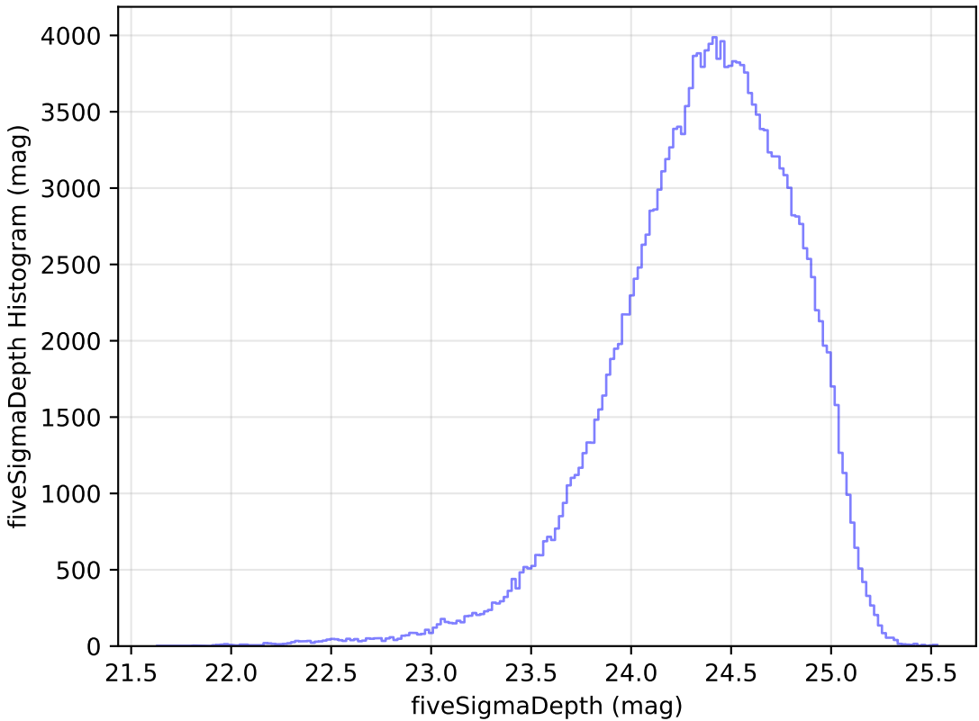
weather_cloudso6v3.4_10yrs g: fiveSigmaDepth Histogram
