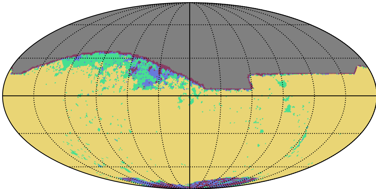
weather_cloudso6v3.4_10yrs z band: YearCoverage night
