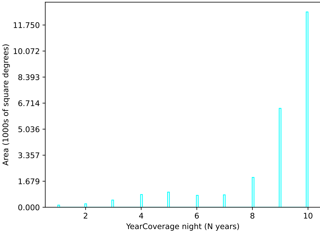
weather_cloudso6v3.4_10yrs u band: YearCoverage night
