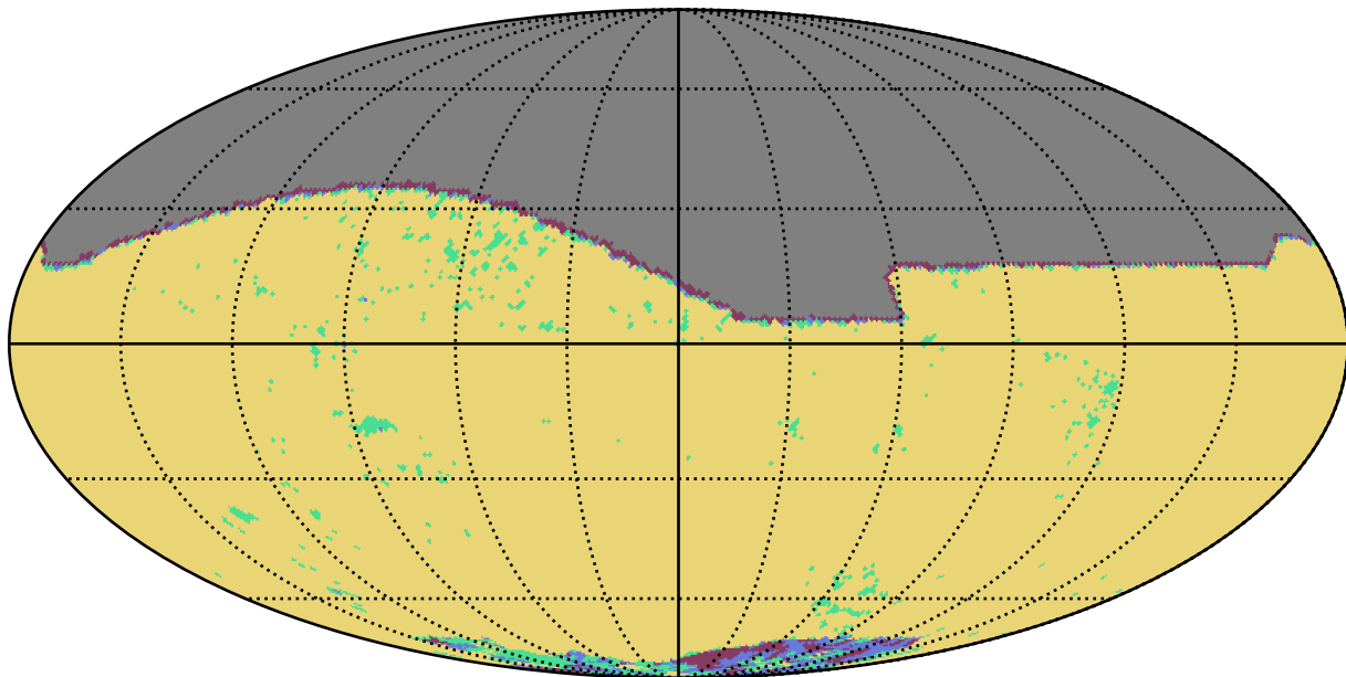
weather_cloudso6v3.4_10yrs r band: YearCoverage night
