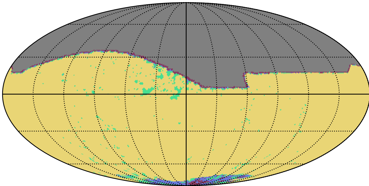
weather_cloudso6v3.4_10yrs i band: YearCoverage night
