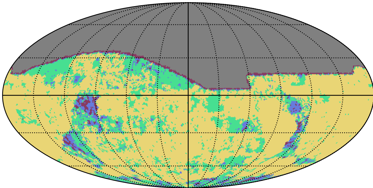
weather_cloudso6v3.4_10yrs g band: YearCoverage night
