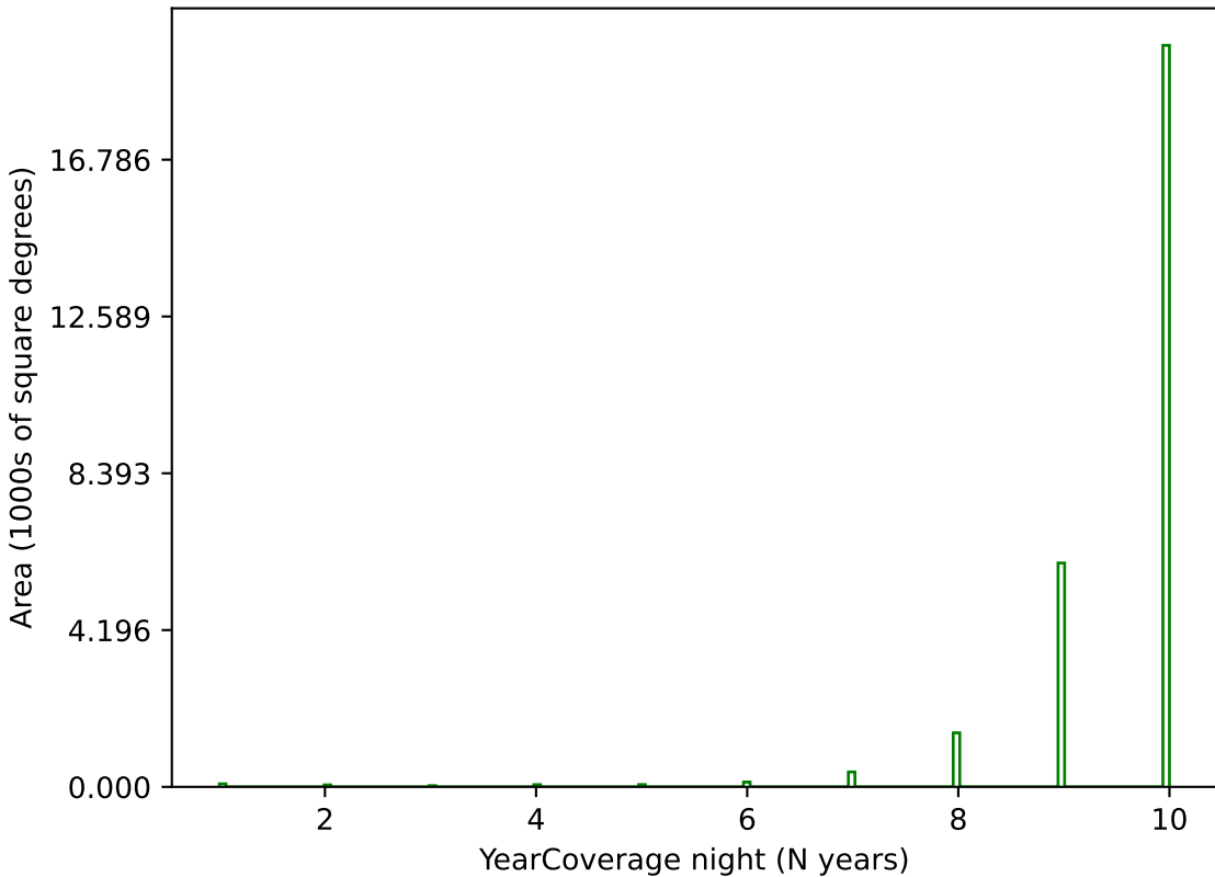
weather_cloudso6v3.4_10yrs g band: YearCoverage night
