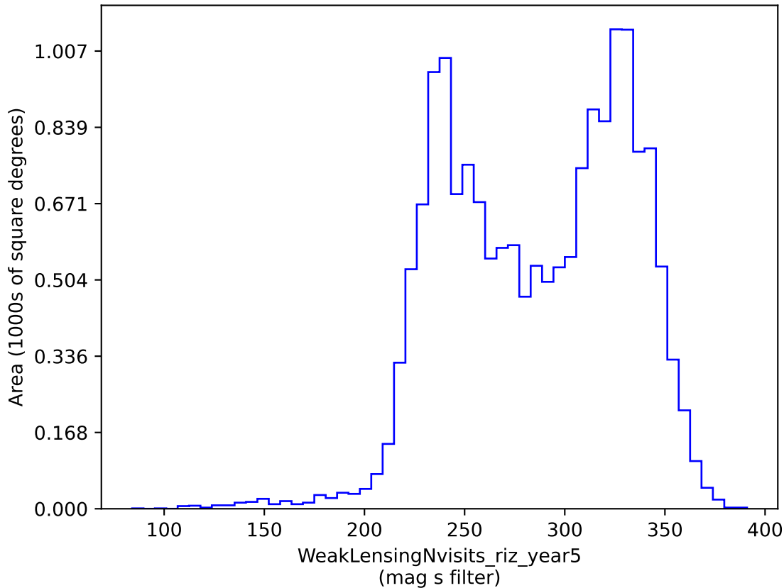
weather_cloudso6v3.4_10yrs gri band non-DD: WeakLensingNvisits_riz_year5
