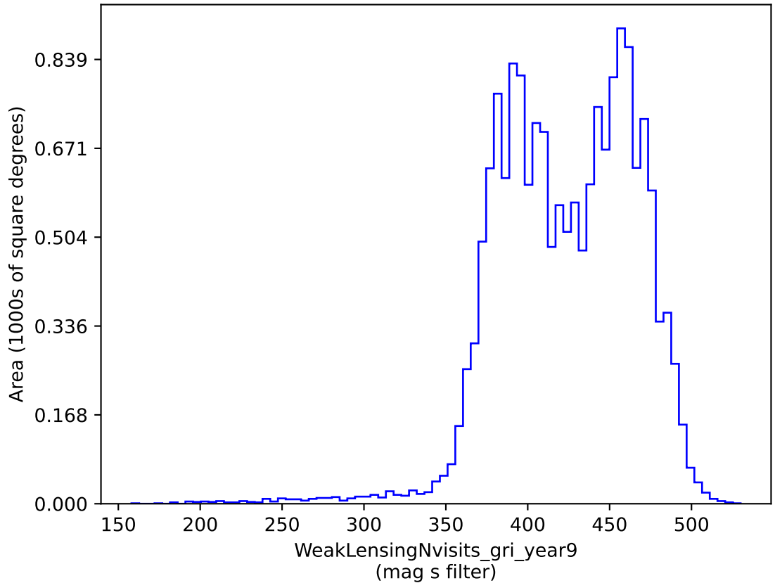
weather_cloudso6v3.4_10yrs gri band non-DD: WeakLensingNvisits_gri_year9
