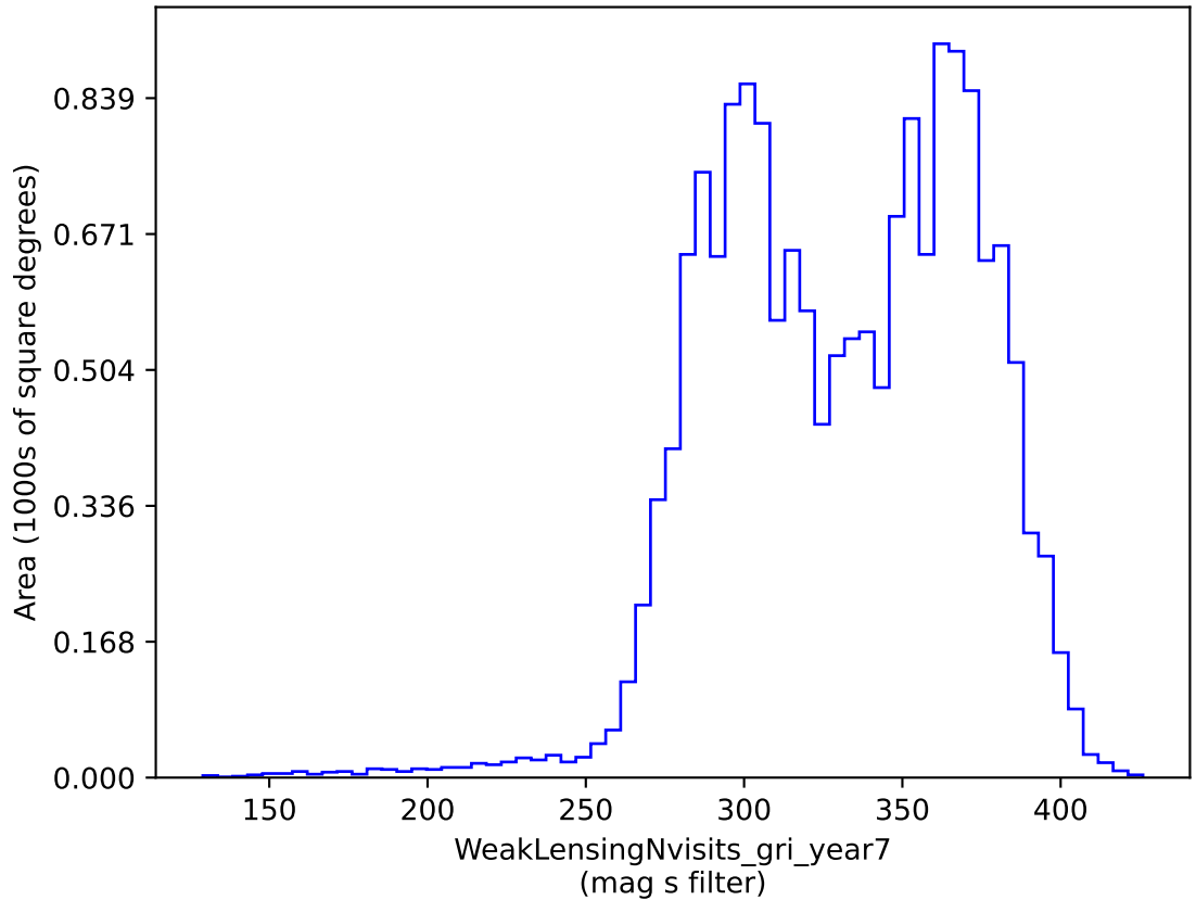
weather_cloudso6v3.4_10yrs gri band non-DD: WeakLensingNvisits_gri_year7
