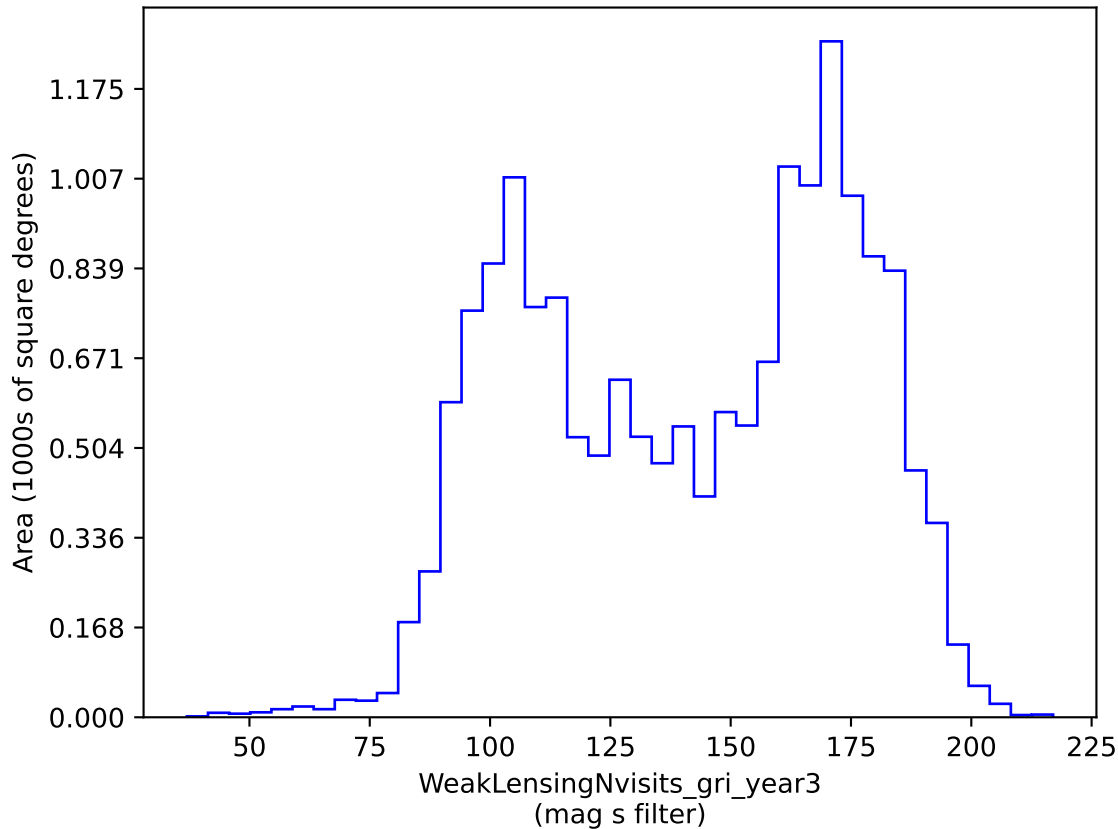
weather_cloudso6v3.4_10yrs gri band non-DD: WeakLensingNvisits_gri_year3
