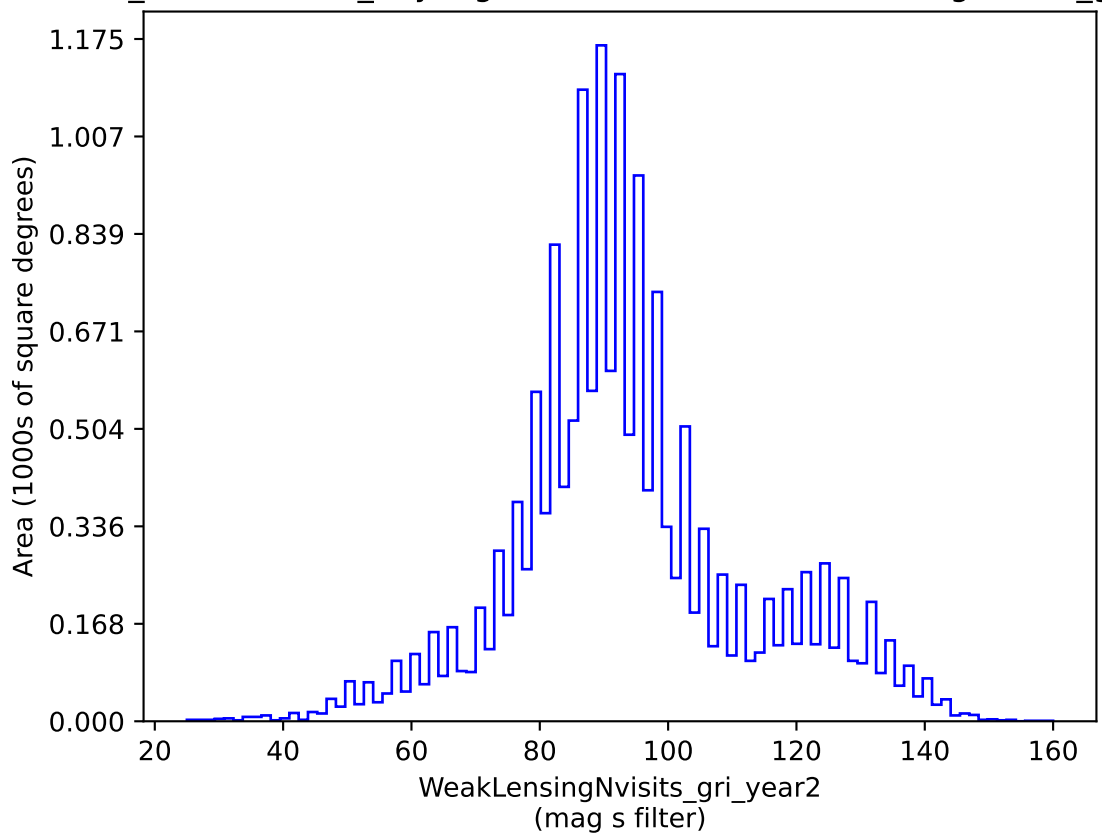
weather_cloudso6v3.4_10yrs gri band non-DD: WeakLensingNvisits_gri_year2
