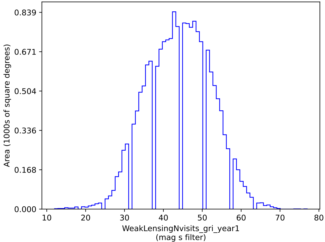
weather_cloudso6v3.4_10yrs gri band non-DD: WeakLensingNvisits_gri_year1
