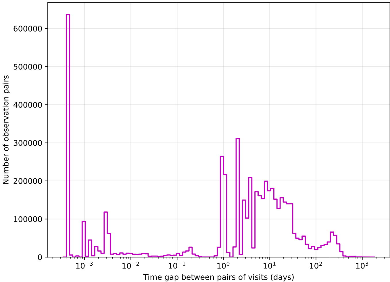
weather_cloudso6v3.4_10yrs z band: Tgaps observationStartMJD
