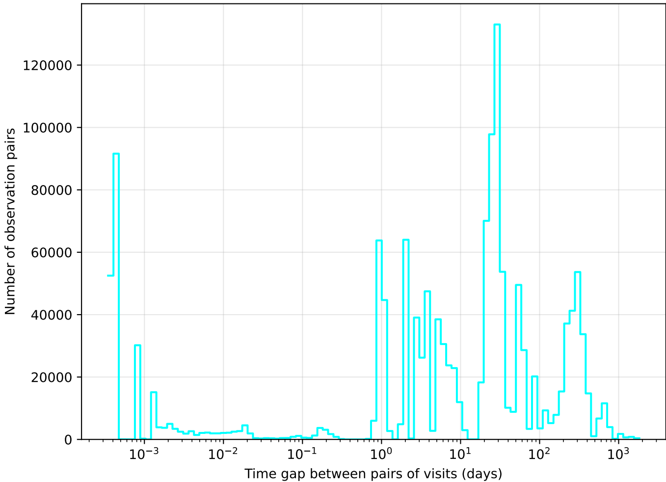
weather_cloudso6v3.4_10yrs u band: Tgaps observationStartMJD
