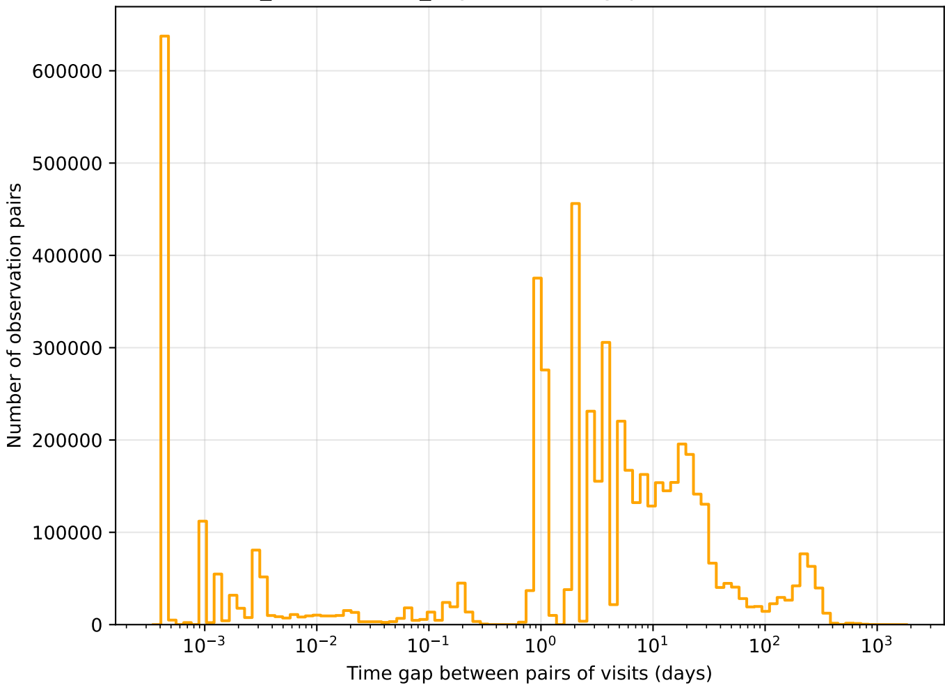
weather_cloudso6v3.4_10yrs r band: Tgaps observationStartMJD
