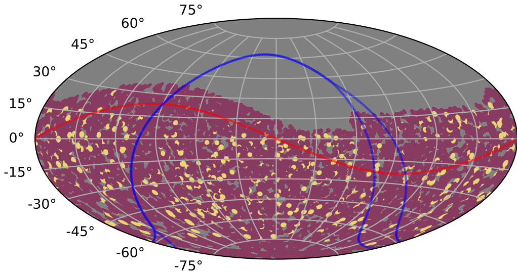
weather_cloudso6v3.4_10yrs : TDEsPopMetric_some_color
