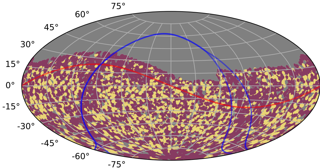
weather_cloudso6v3.4_10yrs : TDEsPopMetric_prepeak
