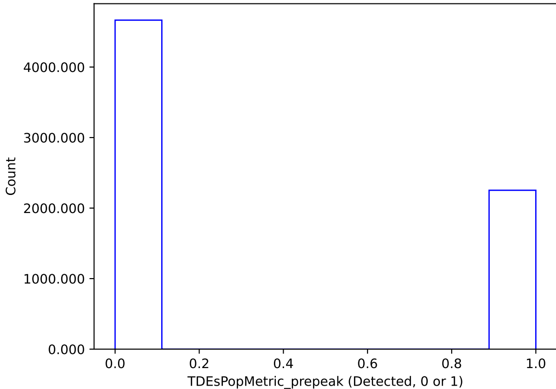
weather_cloudso6v3.4_10yrs : TDEsPopMetric_prepeak
