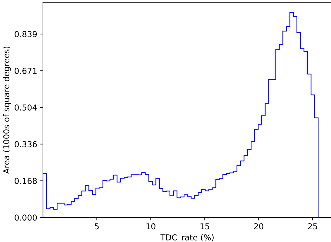
weather_cloudso6v3.4_10yrs : TDC_rate
