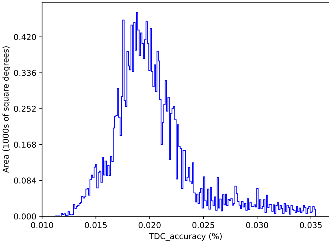
weather_cloudso6v3.4_10yrs : TDC_accuracy
