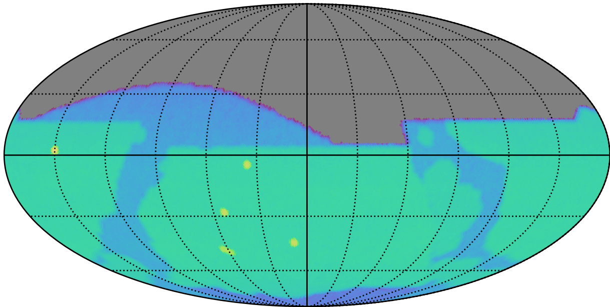
weather_cloudso6v3.4_10yrs z: SurfaceBrightLimit
