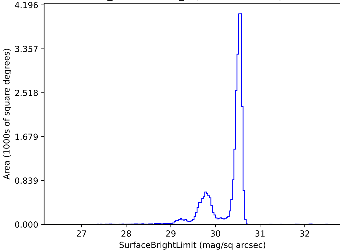
weather_cloudso6v3.4_10yrs r: SurfaceBrightLimit
