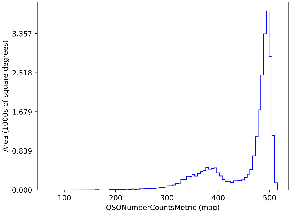
weather_cloudso6v3.4_10yrs z band and non-DD: QSONumberCountsMetric
