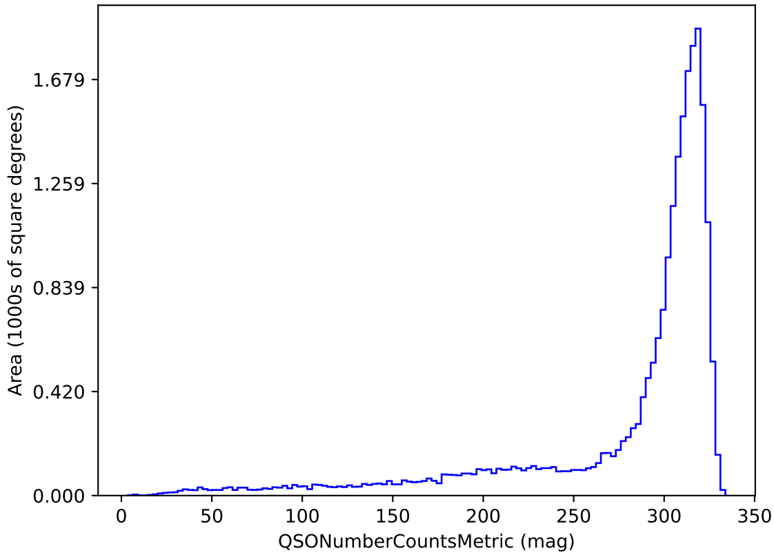
weather_cloudso6v3.4_10yrs u band and non-DD: QSONumberCountsMetric
