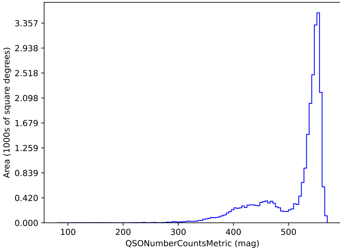
weather_cloudso6v3.4_10yrs i band and non-DD: QSONumberCountsMetric
