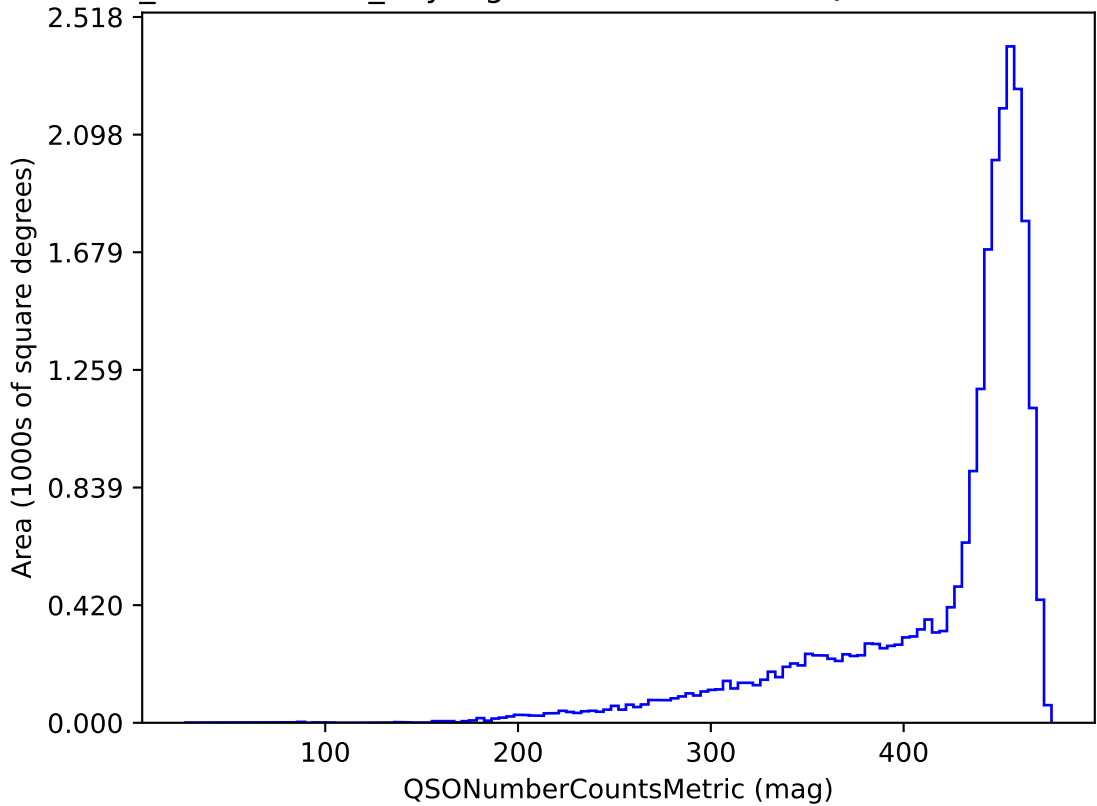
weather_cloudso6v3.4_10yrs g band and non-DD: QSONumberCountsMetric
