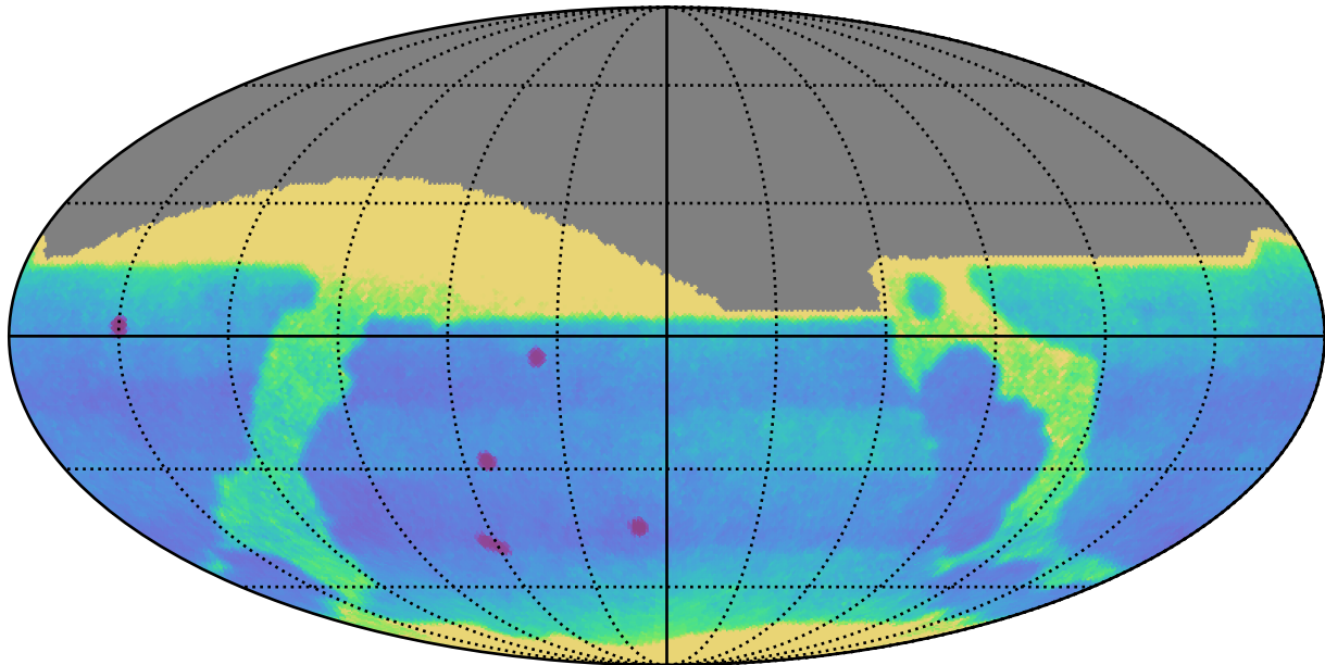
weather_cloudso6v3.4_10yrs : Proper Motion Uncert @ 24.0
