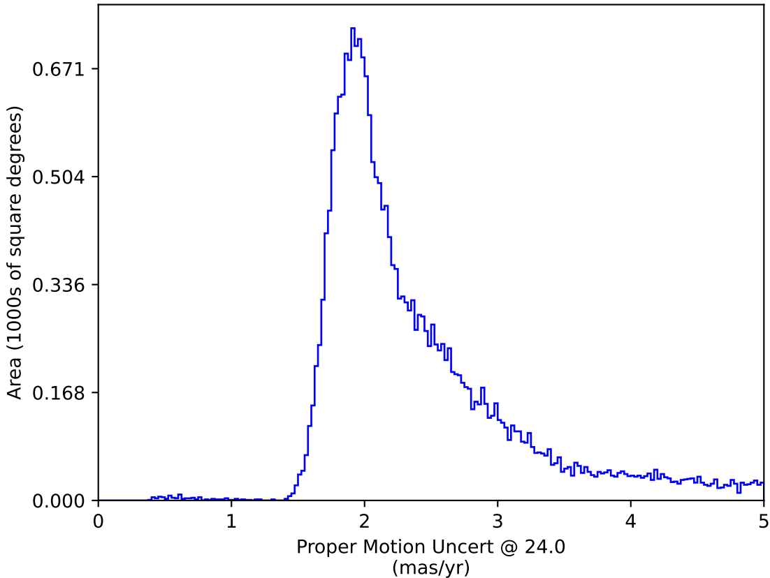
weather_cloudso6v3.4_10yrs : Proper Motion Uncert @ 24.0
