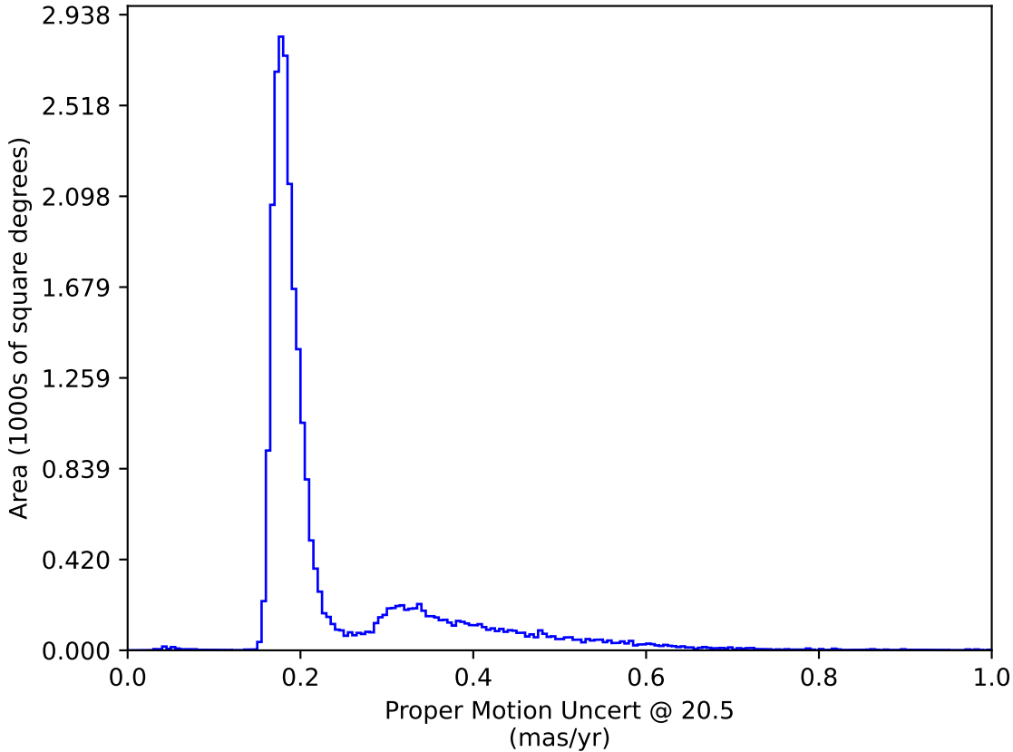
weather_cloudso6v3.4_10yrs : Proper Motion Uncert @ 20.5
