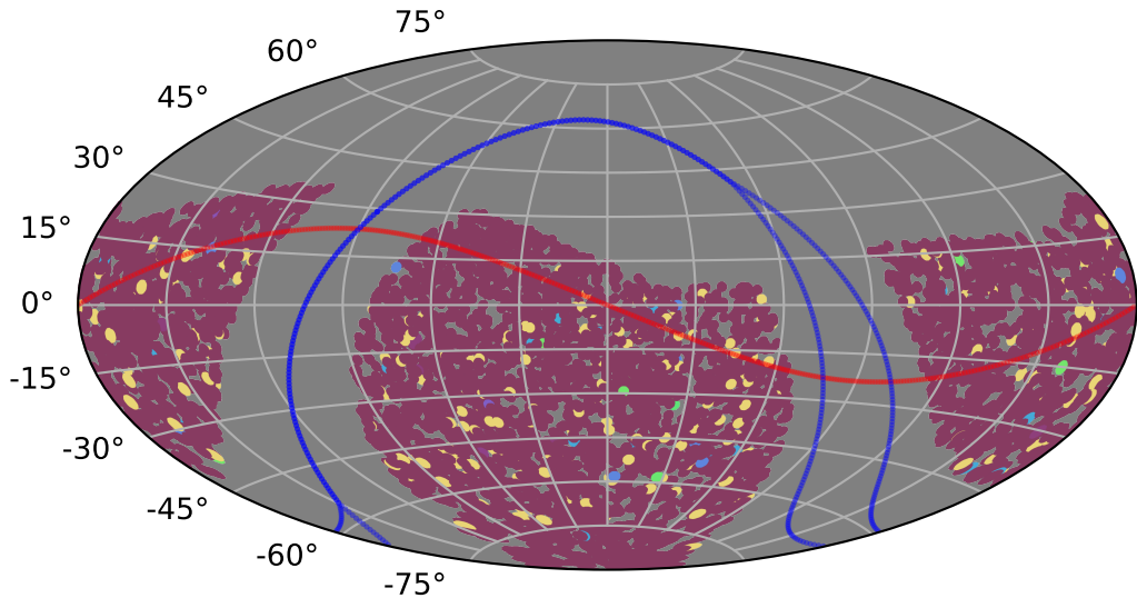
weather_cloudso6v3.4_10yrs : PrestoKNe_score_p
