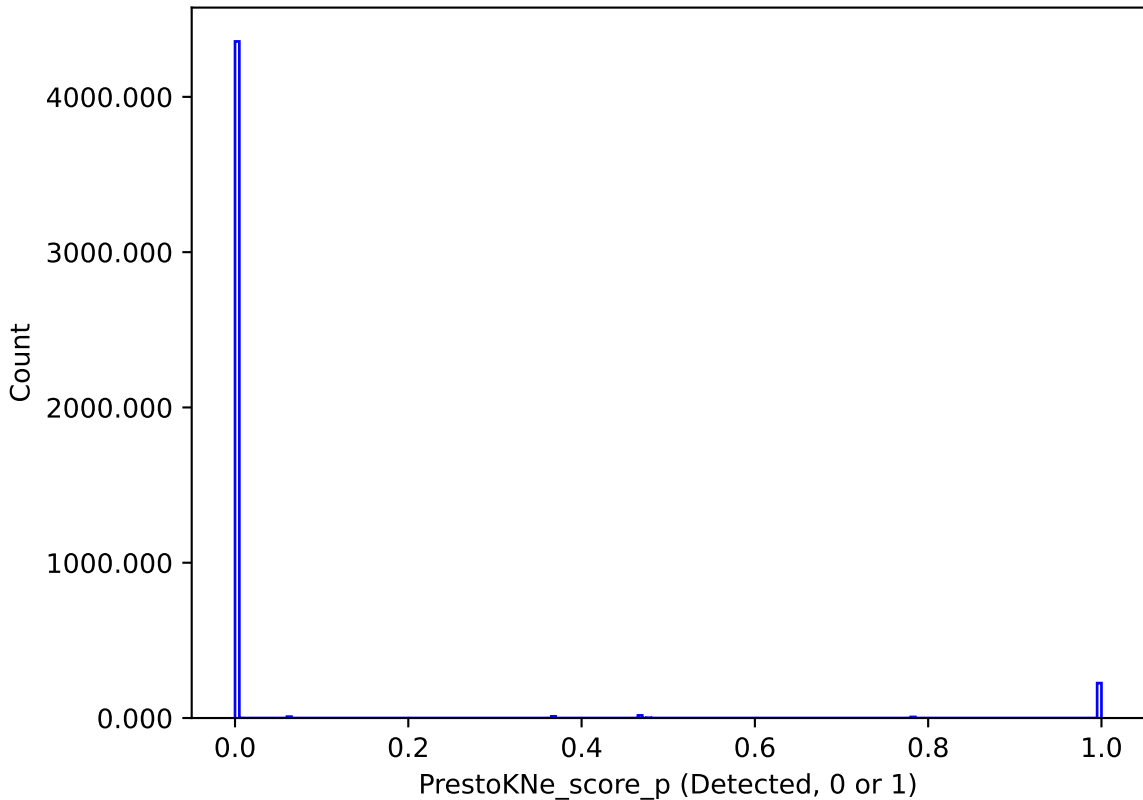
weather_cloudso6v3.4_10yrs : PrestoKNe_score_p
