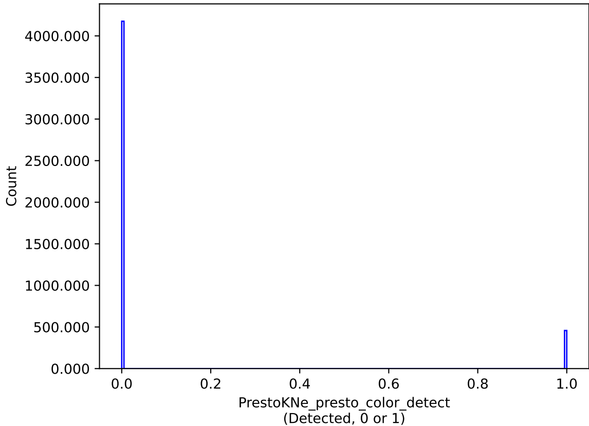
weather_cloudso6v3.4_10yrs : PrestoKNe_presto_color_detect
