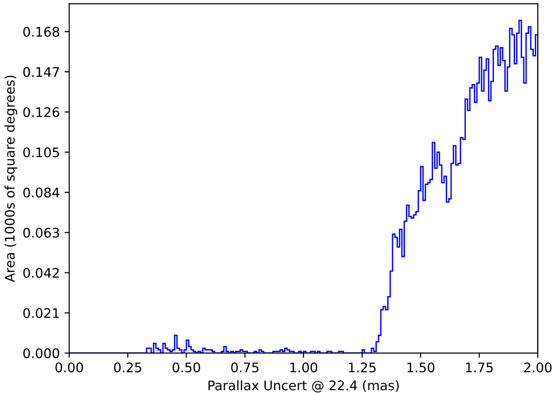
weather_cloudso6v3.4_10yrs : Parallax Uncert @ 22.4
