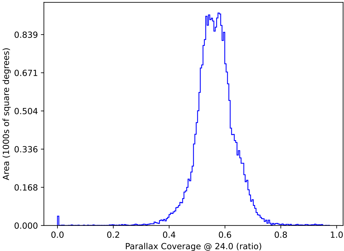
weather_cloudso6v3.4_10yrs : Parallax Coverage @ 24.0
