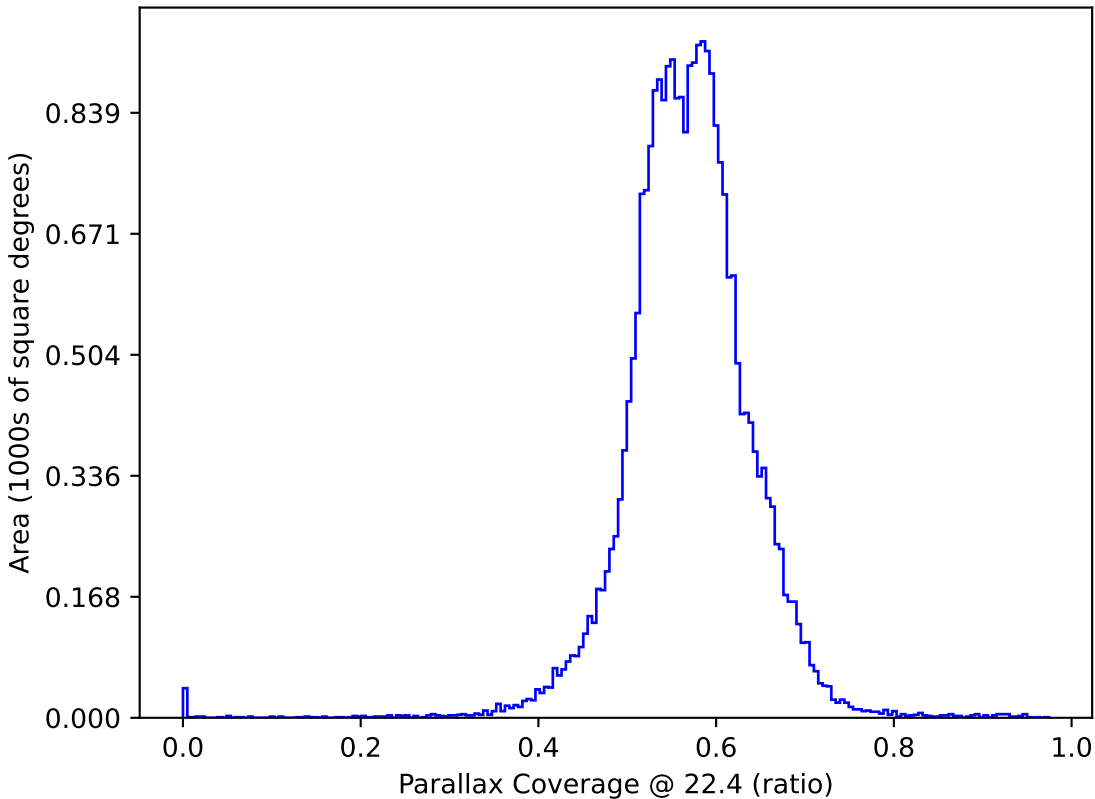
weather_cloudso6v3.4_10yrs : Parallax Coverage @ 22.4
