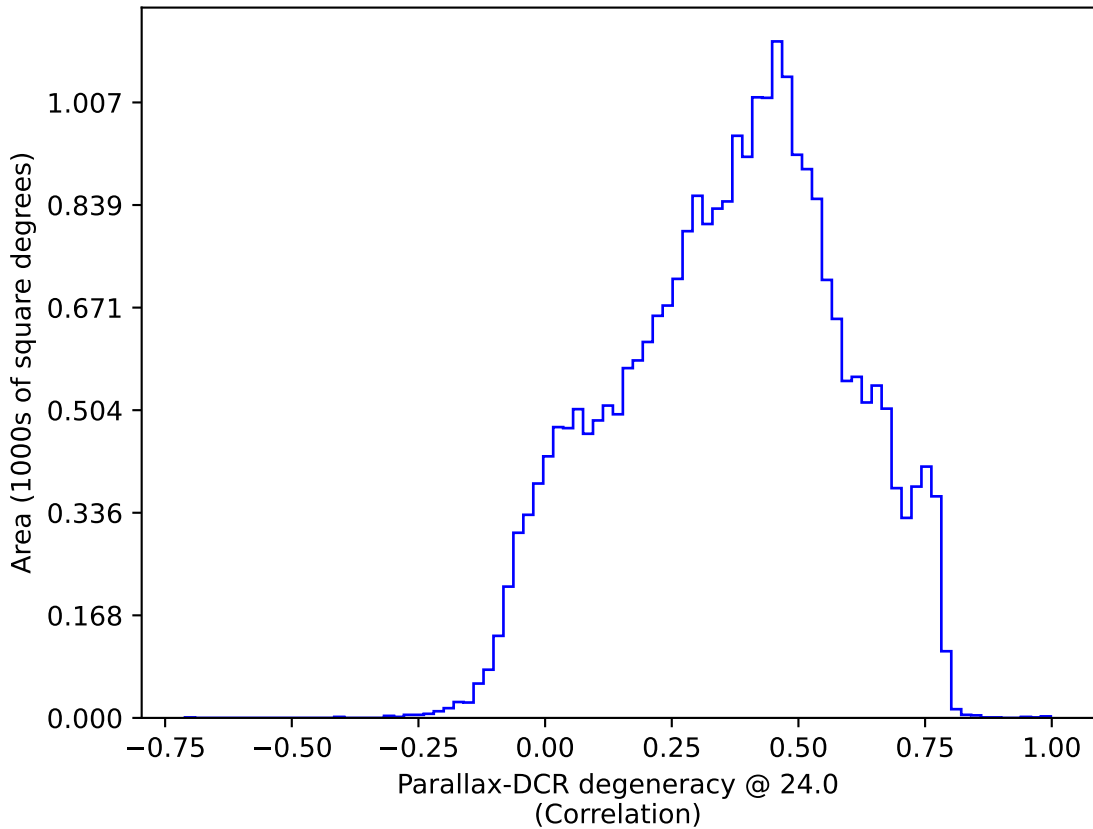
weather_cloudso6v3.4_10yrs : Parallax-DCR degeneracy @ 24.0
