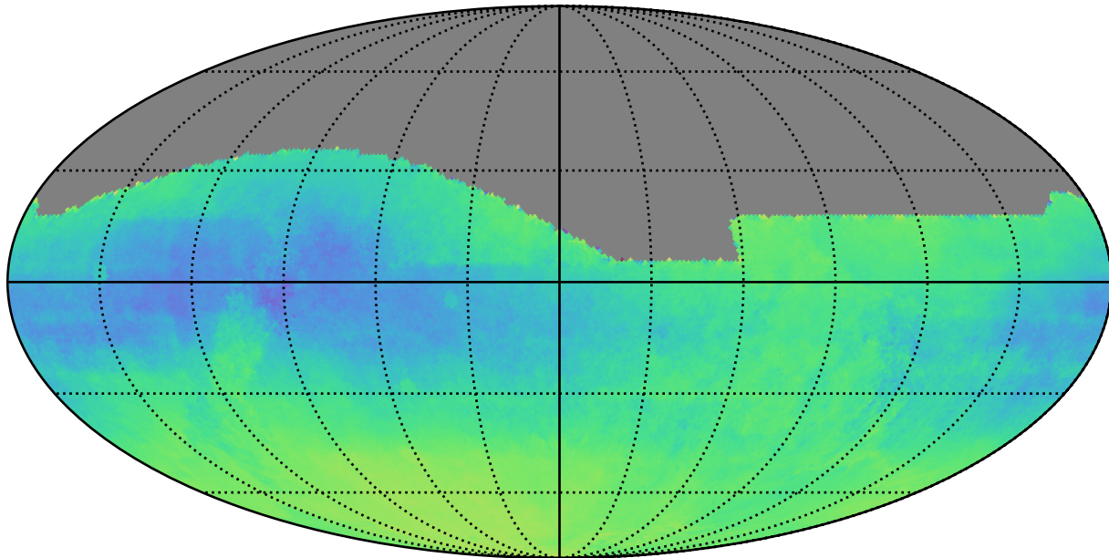
weather_cloudso6v3.4_10yrs : Parallax-DCR degeneracy @ 22.4
