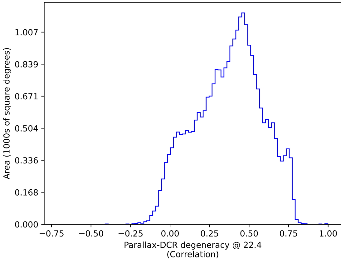
weather_cloudso6v3.4_10yrs : Parallax-DCR degeneracy @ 22.4
