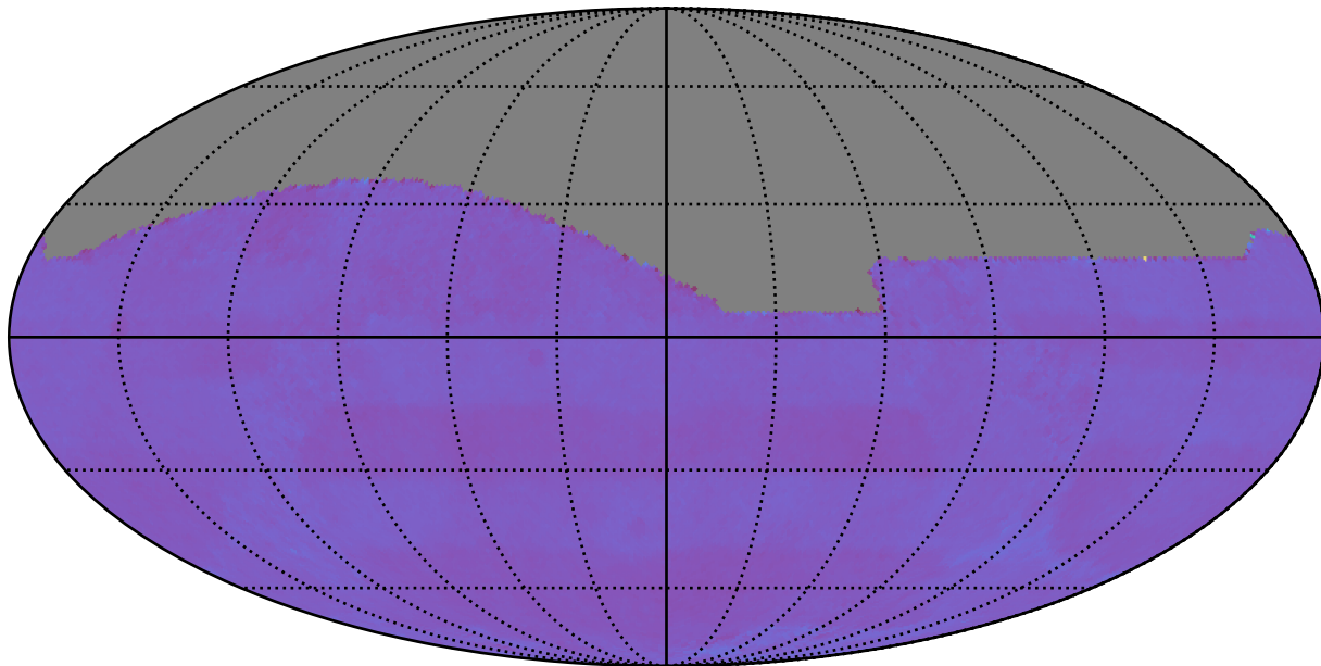
weather_cloudso6v3.4_10yrs : Normalized Proper Motion Uncert @ 24.0
