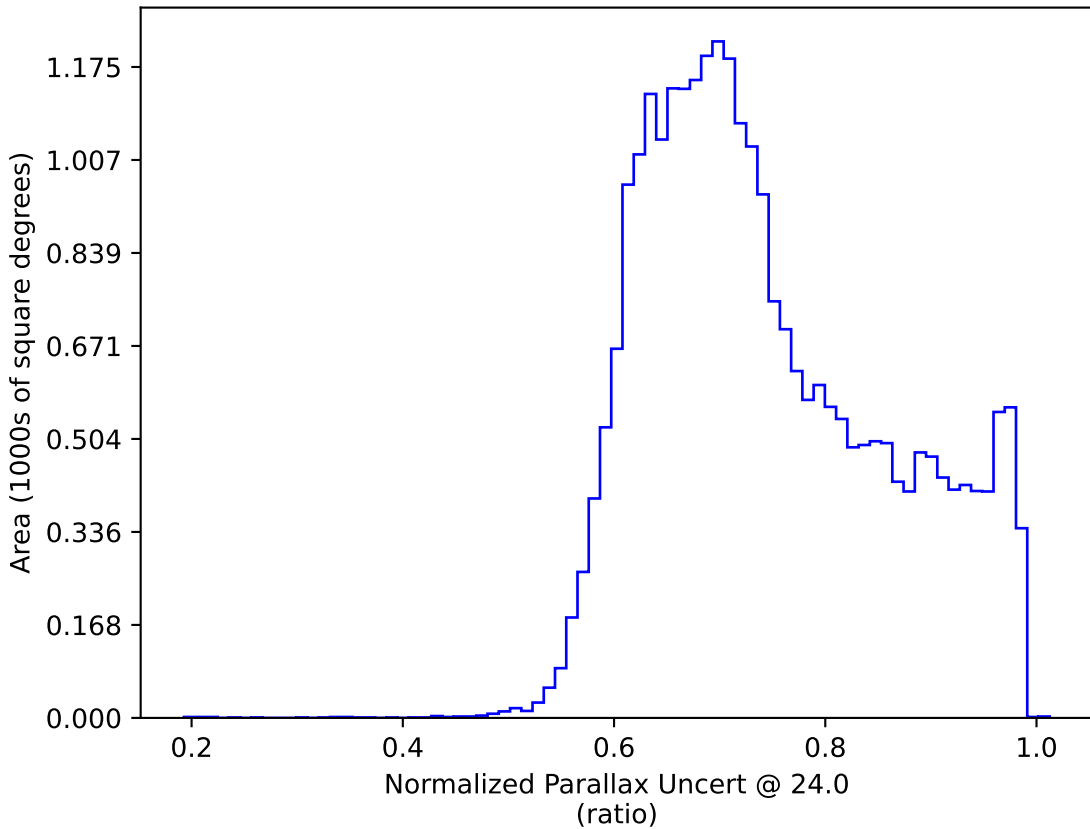
weather_cloudso6v3.4_10yrs : Normalized Parallax Uncert @ 24.0
