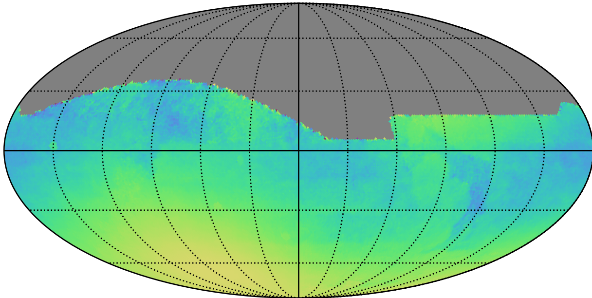
weather_cloudso6v3.4_10yrs : Normalized Parallax Uncert @ 22.4
