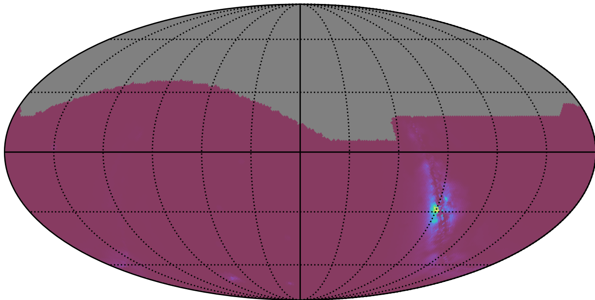
weather_cloudso6v3.4_10yrs : NlcPoints
