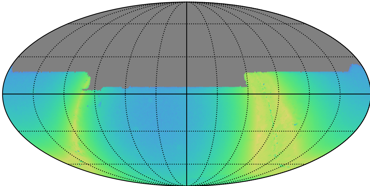
weather_cloudso6v3.4_10yrs y: N stars to Precision 0.20
