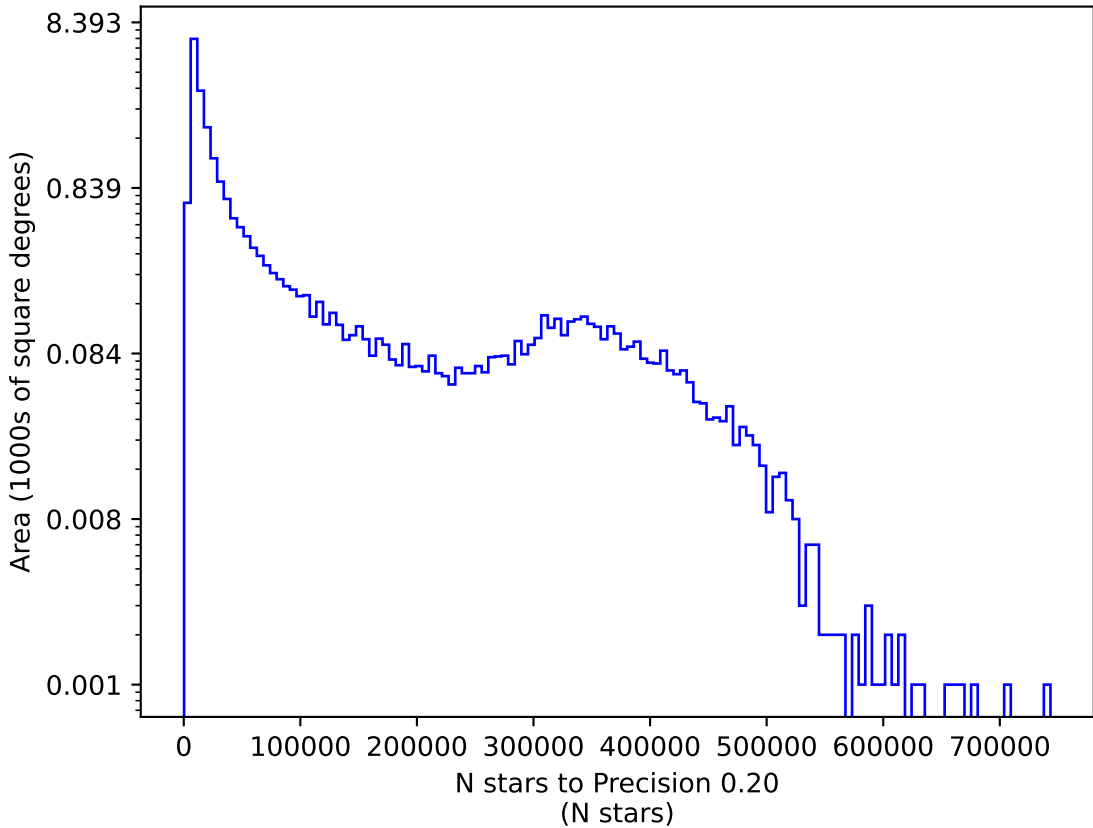
weather_cloudso6v3.4_10yrs y: N stars to Precision 0.20
