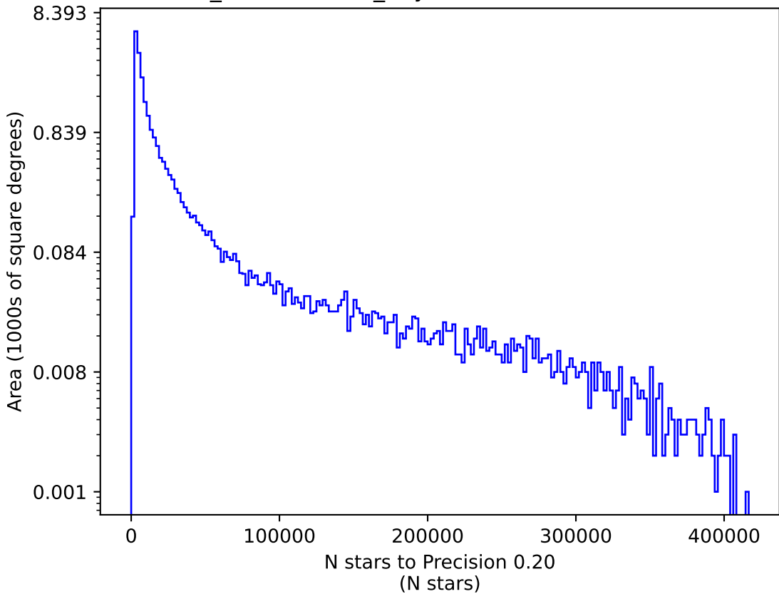
weather_cloudso6v3.4_10yrs u: N stars to Precision 0.20
