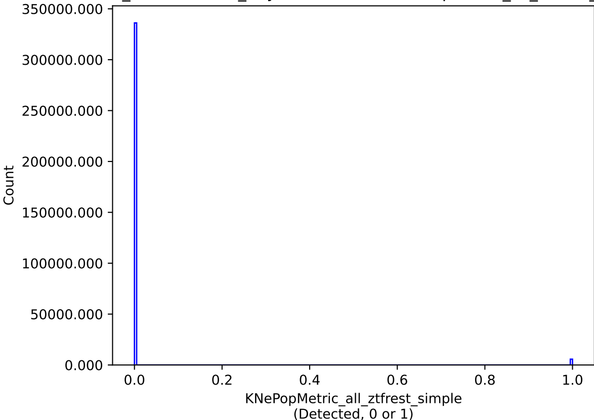
weather_cloudso6v3.4_10yrs all models: KNePopMetric_all_ztfrest_simple
