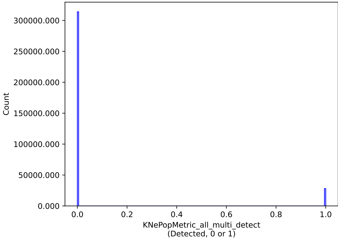
weather_cloudso6v3.4_10yrs all models: KNePopMetric_all_multi_detect
