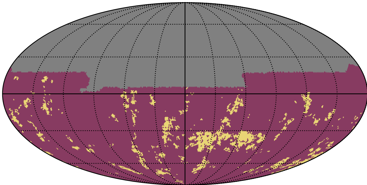
weather_cloudso6v3.4_10yrs u band: Gaps_7hr
